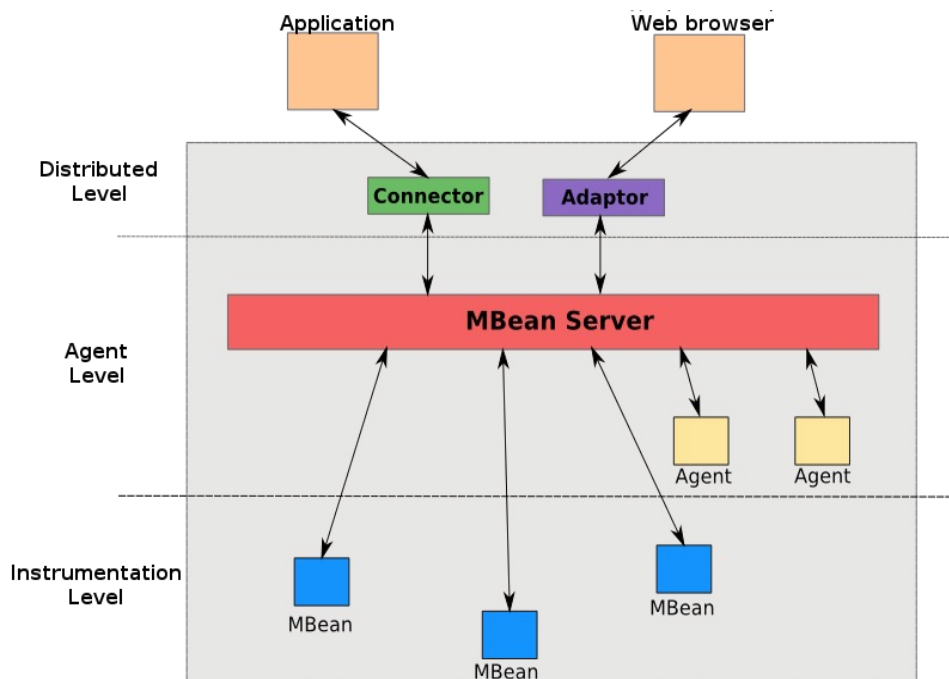
Illustration 1: Architecture JMX
